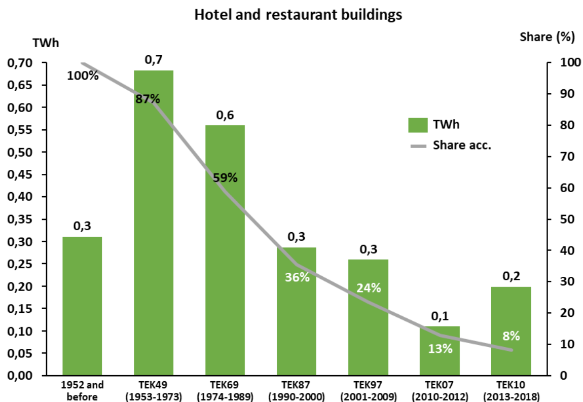
Figure 25 Share energy demand related to hotel and restaurant buildings depending on building year
